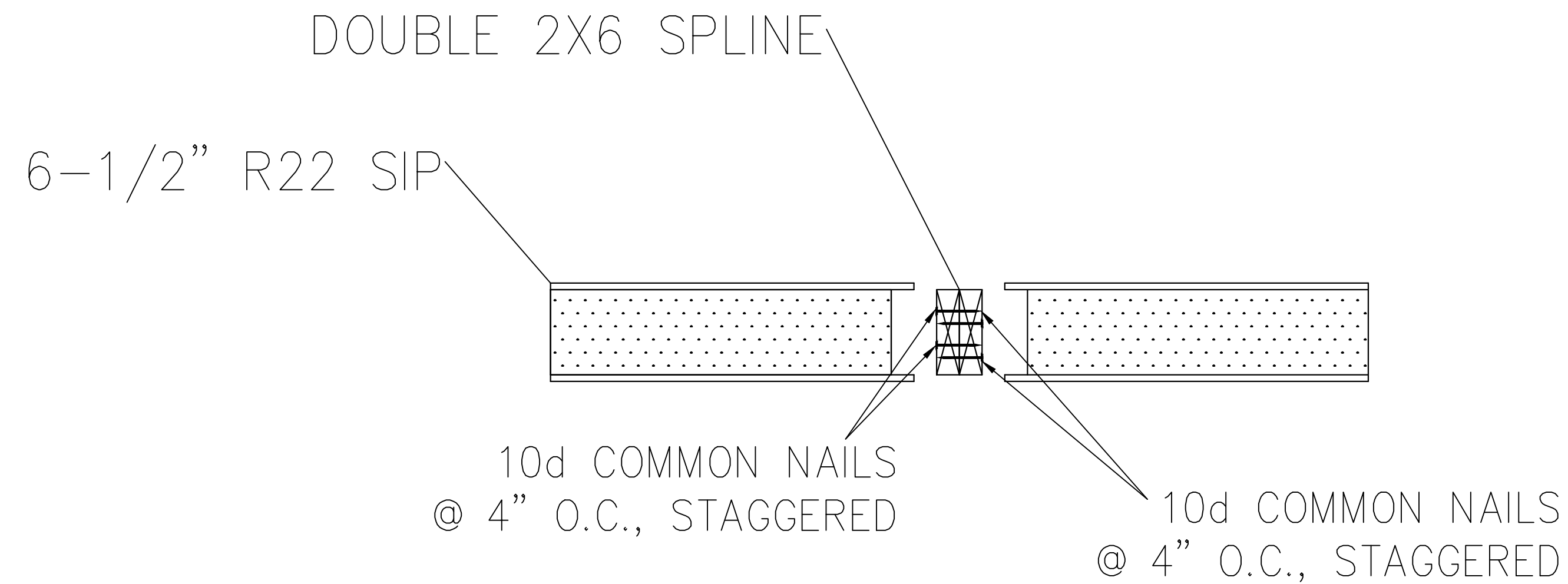
DOUBLE 2X6 WALL SIP SPLINE CONNECTION
