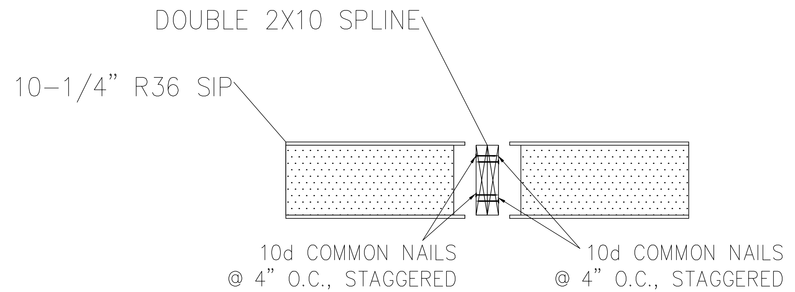
DOUBLE 2X10 ROOF SPLINE CONNECTION
