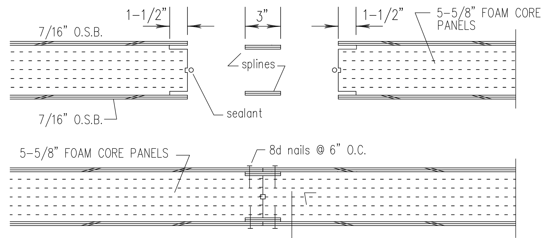
WALL SIP SPLINE CONNECTION
