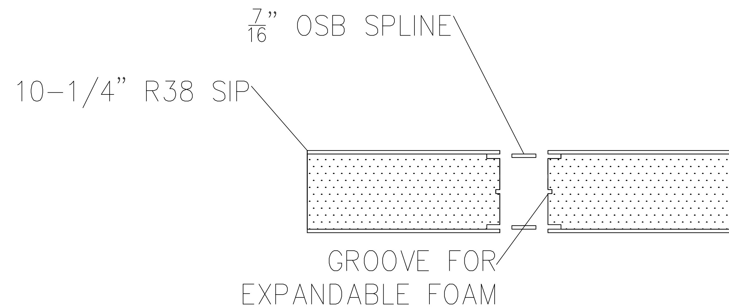
ROOF SIP DOUBLE SPLINE CONNECTION
