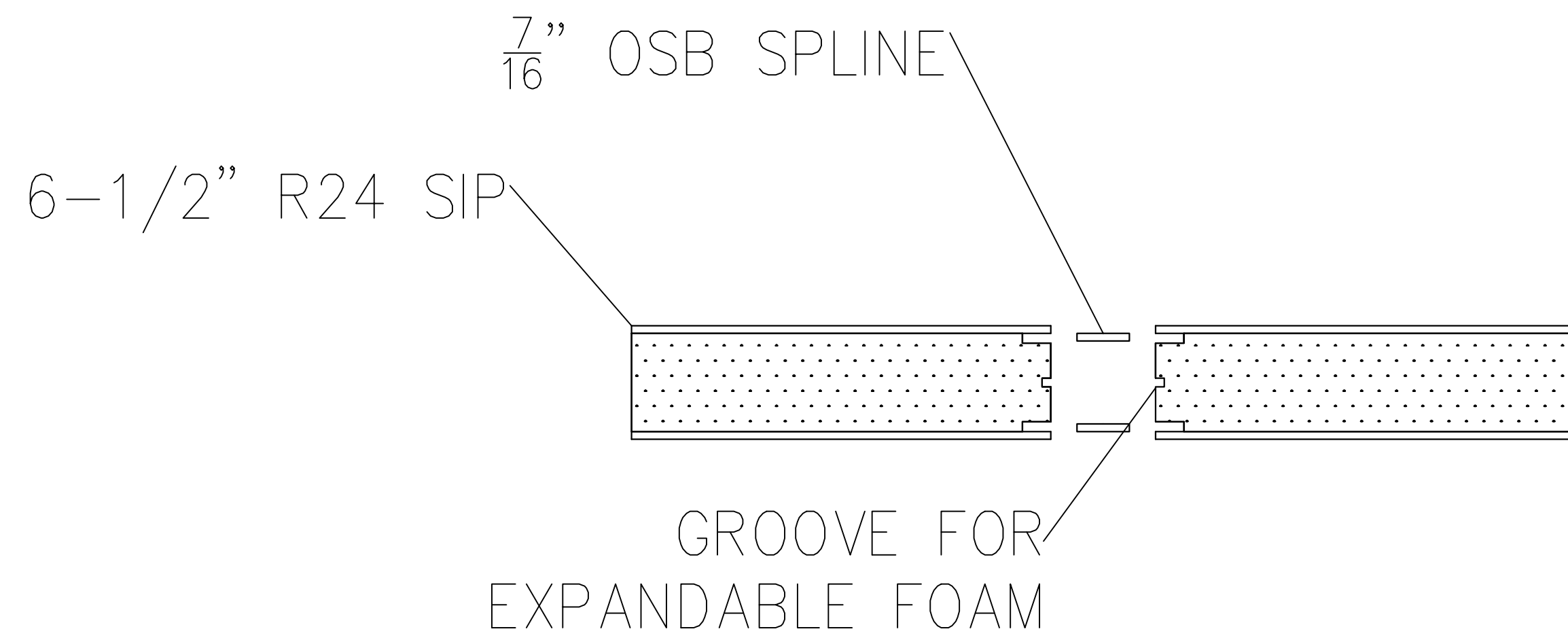
WALL SIP SPLINE CONNECTION
